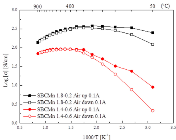
Fig. 4. Dependence of SBCMn electrical conductivity on Mn substitution
