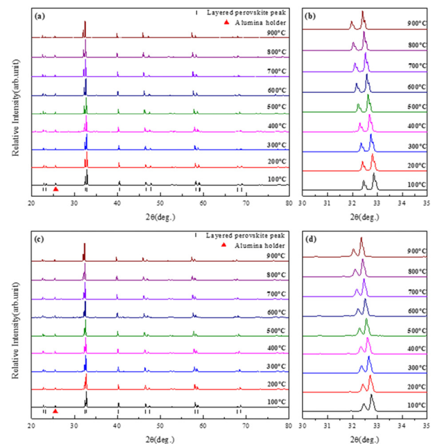
Fig. 2. In-situ XRD patterns of (a) SBCMn 1.8-0.2 (20~80°), (b) SBCMn 1.8-0.2 (30~35°), (c) SBCMn 1.4-0.6 (20~80°), (d) SBCMn 1.4-0.6 (30~35°)
