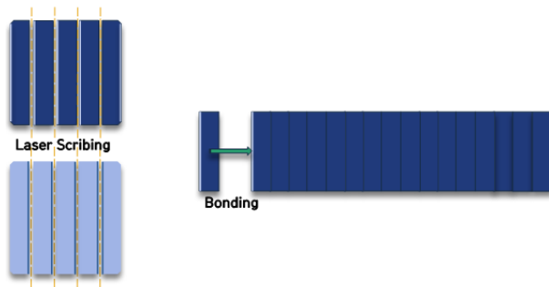
Fig. 1. The process of making a shingled string with shingled cells
