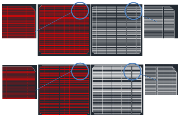
Fig. 2. Different electrode structure forms of ordinary (a) bifacial cells and (b) shingled bifacial cells
