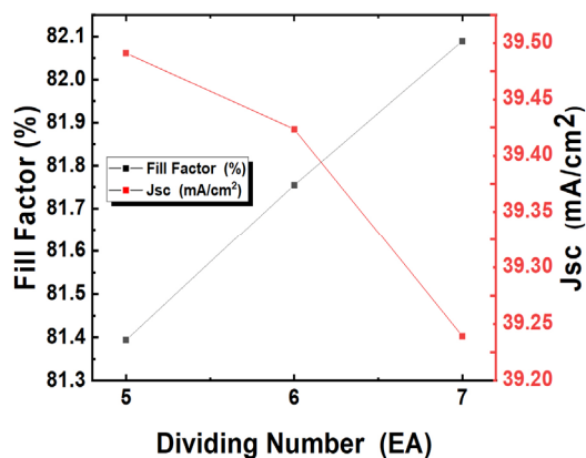
Fig. 4. Changes in J_{sc} and FF according to M6 divisions
