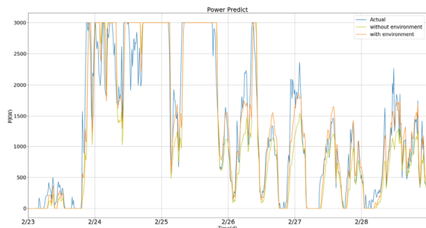
Fig. 10. Comparison curve for prediction accuracy
