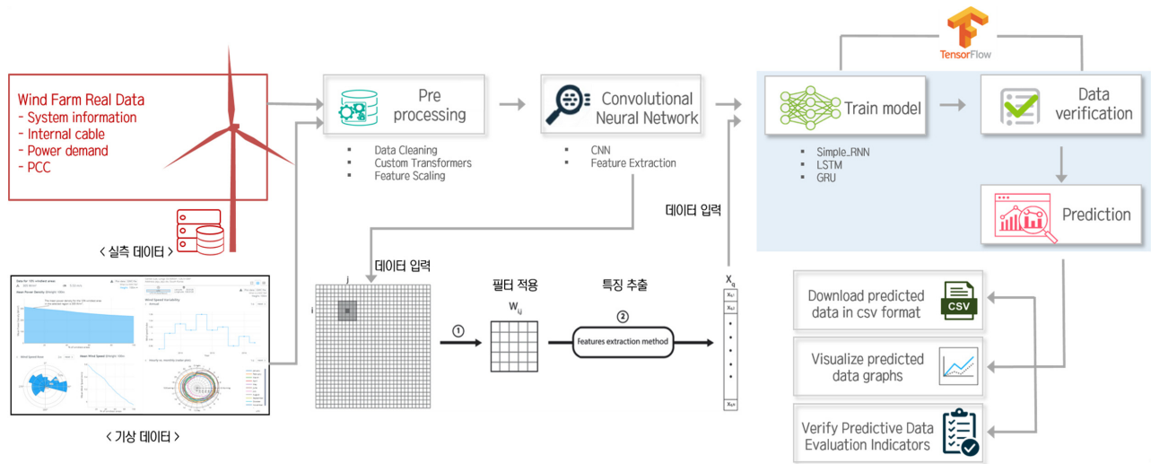
Fig. 1. Configuration of wind power prediction system
