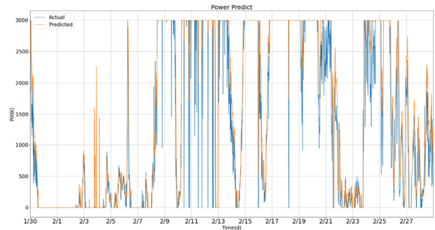
Fig. 7. Prediction curve without CNN
