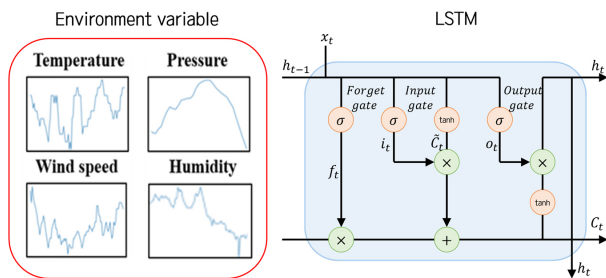
Fig. 5. LSTM configuration
