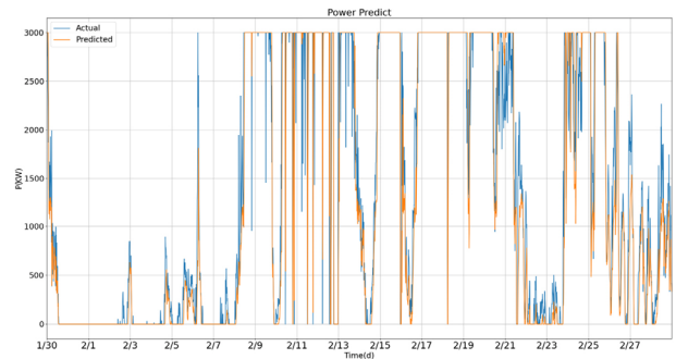
Fig. 8. Prediction curve with no environmental factors
