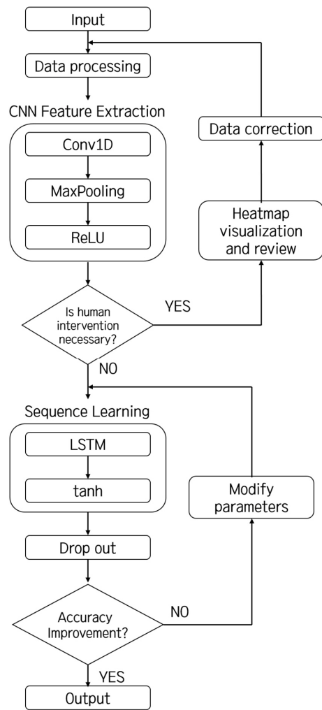
Fig. 6. Proposed flow chart for prediction
