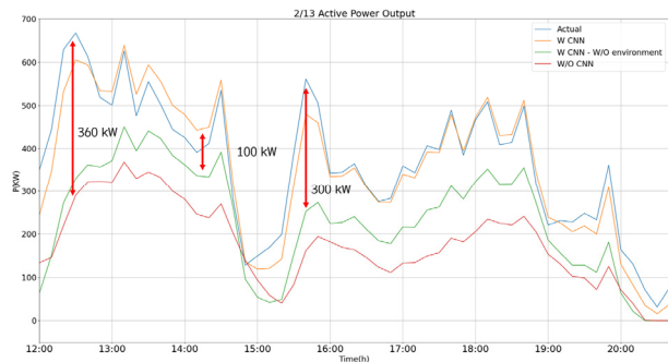
Fig. 11. Closed comparison curve for prediction accuracy
