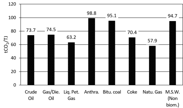
Fig. 9. The CO 2 reduction effect of each major 1 st fossil fuel energy by unit TJ production
