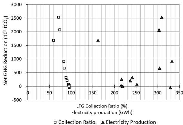
Fig. 8. The relations of LFG collection ratio and electricity generation to Net tCO 2 reduction
